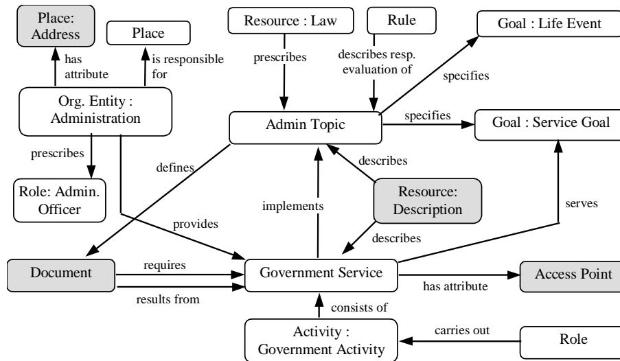
Fig. 3. Fragment of ontology-like structure, as it was identified for the Access-eGov system
