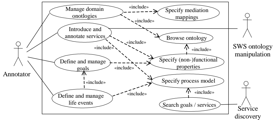
Fig. 2. Use-case diagram for the process of semantic annotation
